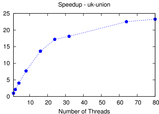
Figure 3. Speedup of the parallel MANIS algorithm (i.e., how much faster is running the algorithm on n threads over running it sequentially) as the number of cores used is varied.
