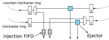
Figure 2: Node router.
