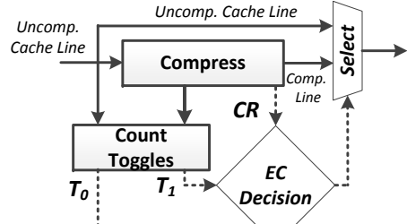
Figure 6. Energy Control decision mechanism.
