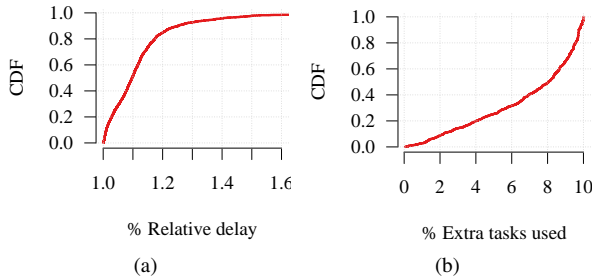
Figure 22: (a) CDF of % time that the job was delayed (b) CDF of % of extra map tasks used.
