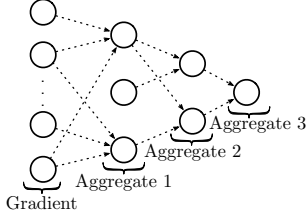
Figure 12: Execution DAG for Stochastic Gradient Descent (SGD).
