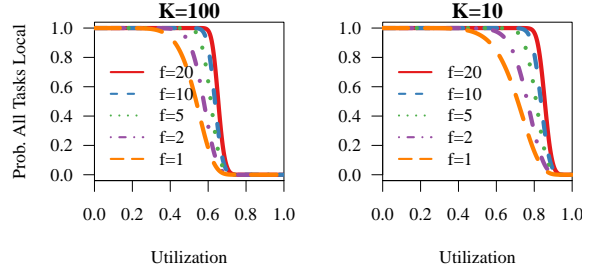
Figure 5: Probability of input-stage locality when using a sampling function which outputs f disjoint samples. Sampling functions specify additional constraints for samples.
